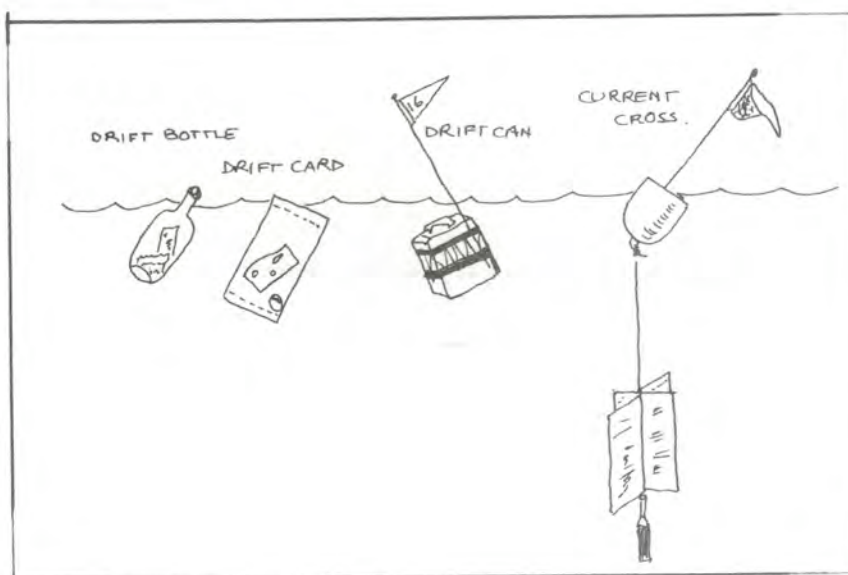
Fig. 10-12: Types of Free Trajectory Current Measuring devices.
