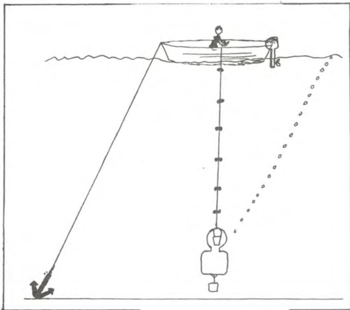
Fig. 10-8: Water Sampling
