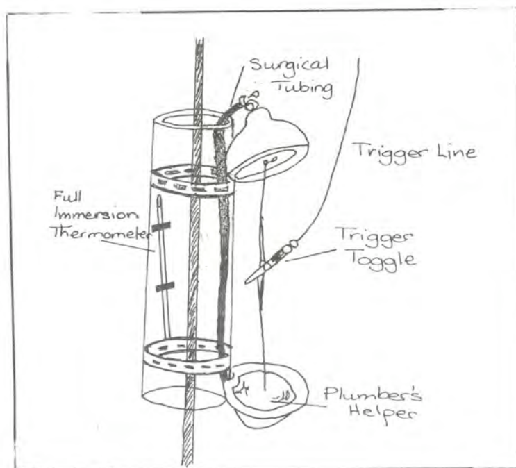
Fig. 10-11: A More Elaborate Water Sampler Bottle.
