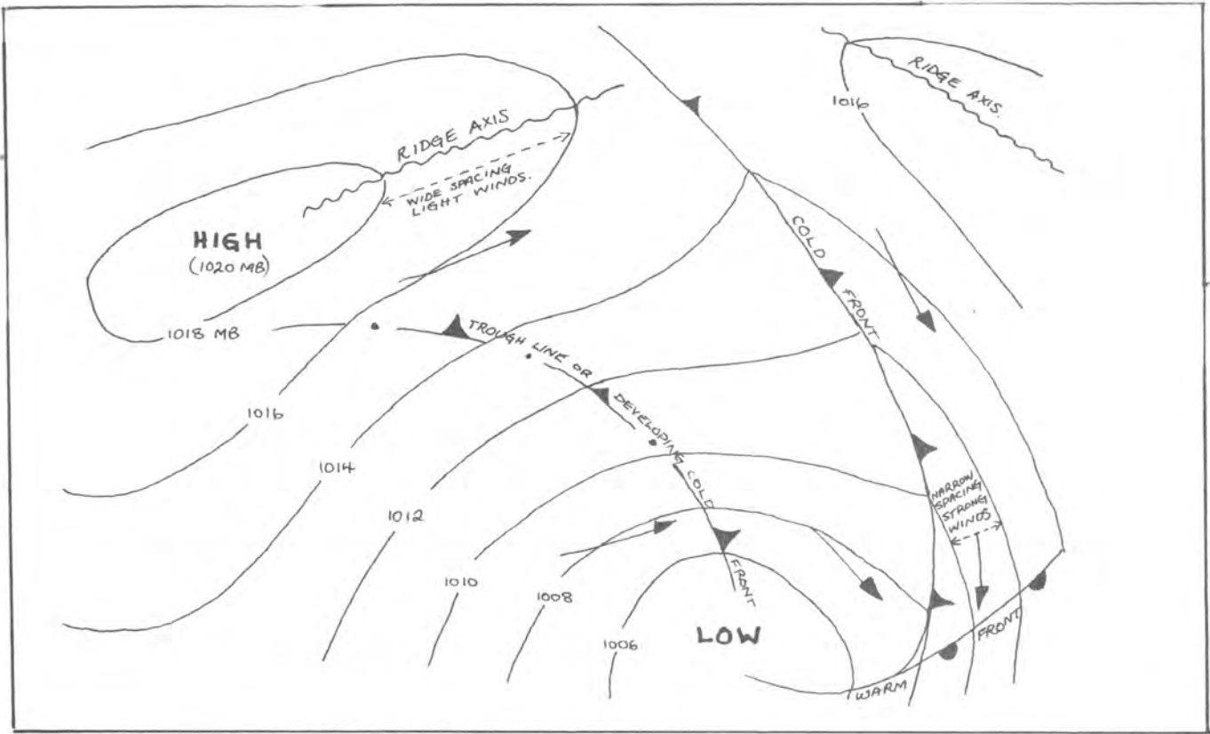
Fig. 10-2: A Typical Weather Map
