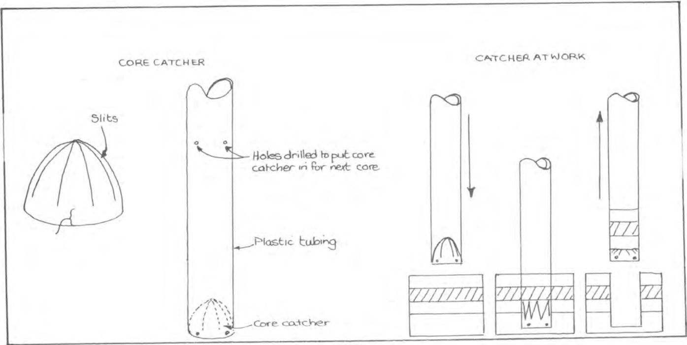
Fig. 10-16: The Hand Corer.
